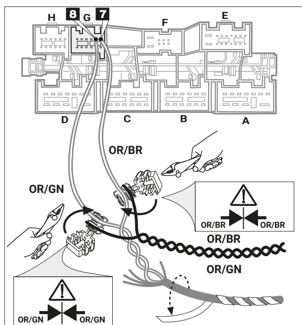
Network control unit position "G" 12 pin connector (BK) chambers 7+8
