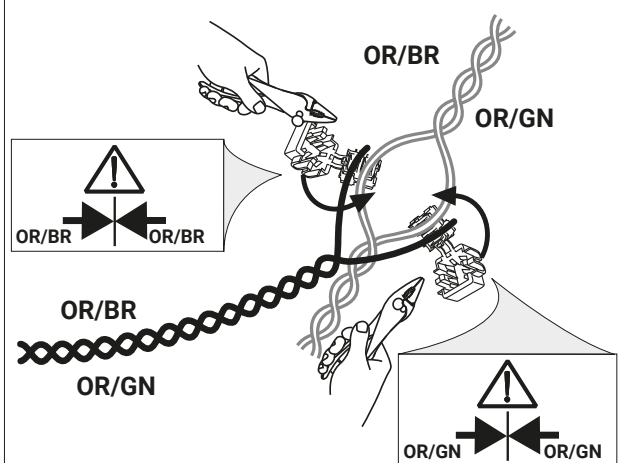
Connector 52-pin (BR)
